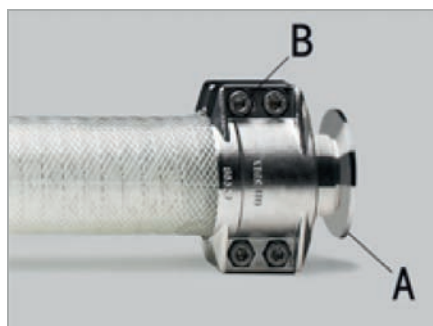
A - STAINLESS STEEL 316 L B - STAINLESS STEEL OR 316 L OR ALUMINIUM
